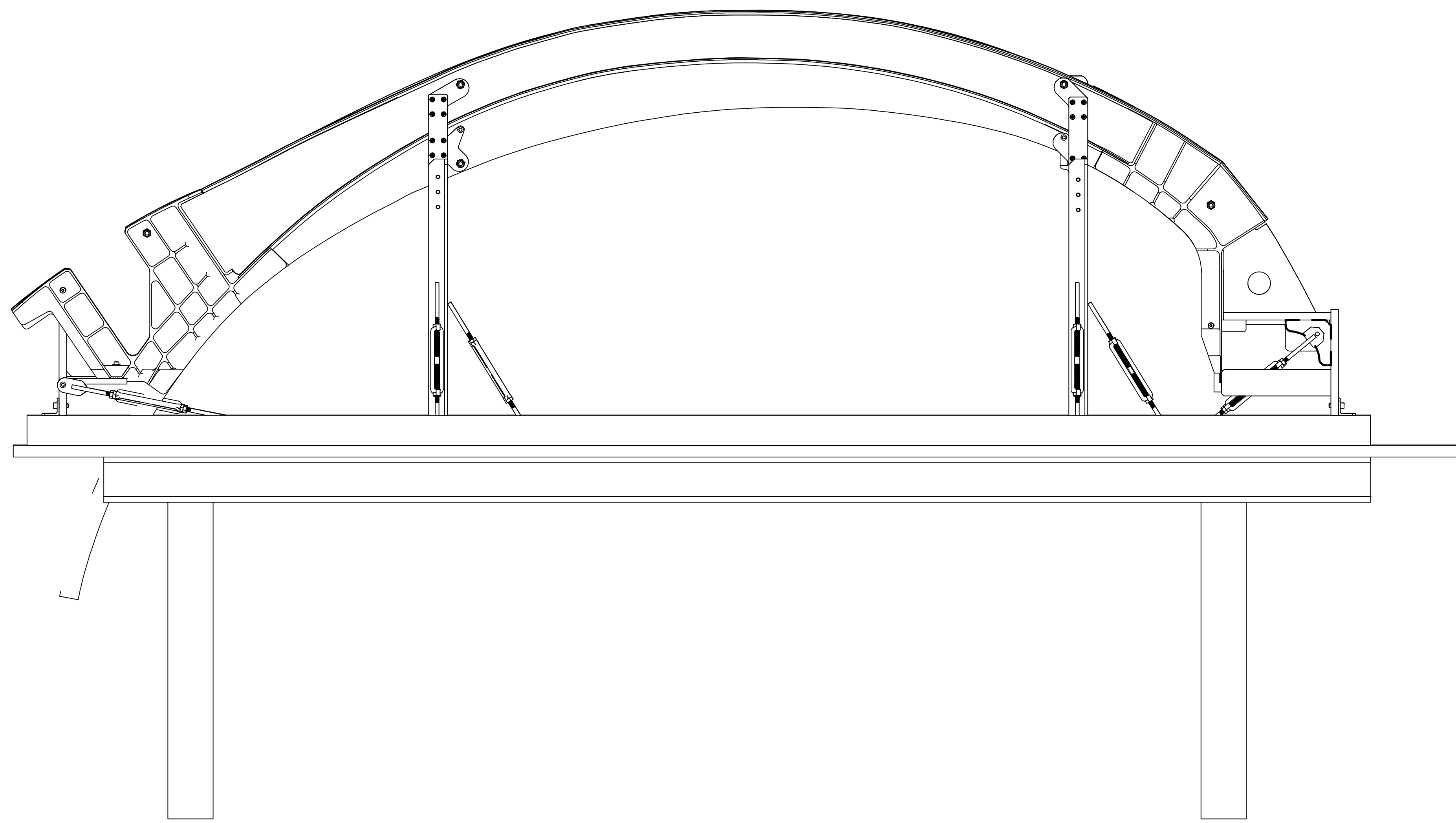
508-1 ASSEMBLY FIXTURE
