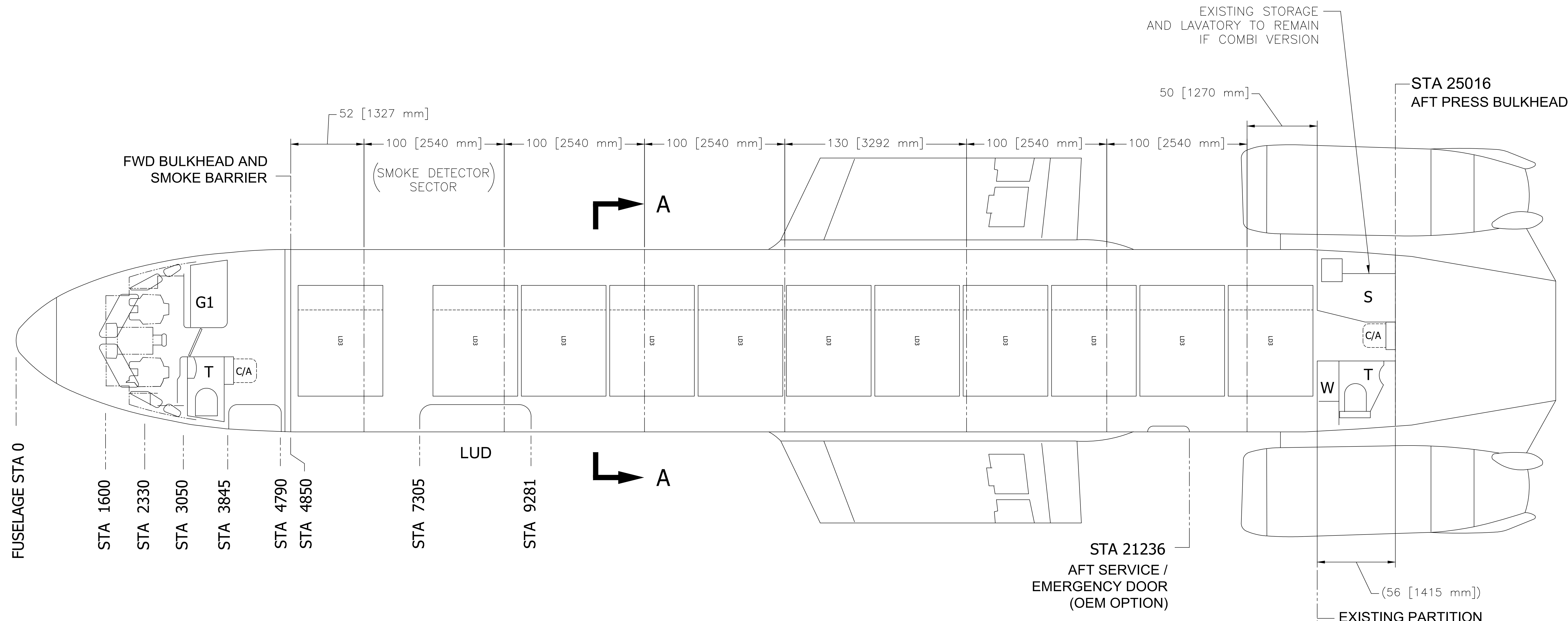
VIEW SHOWING LD3 CONTAINER ARRANGEMENT
