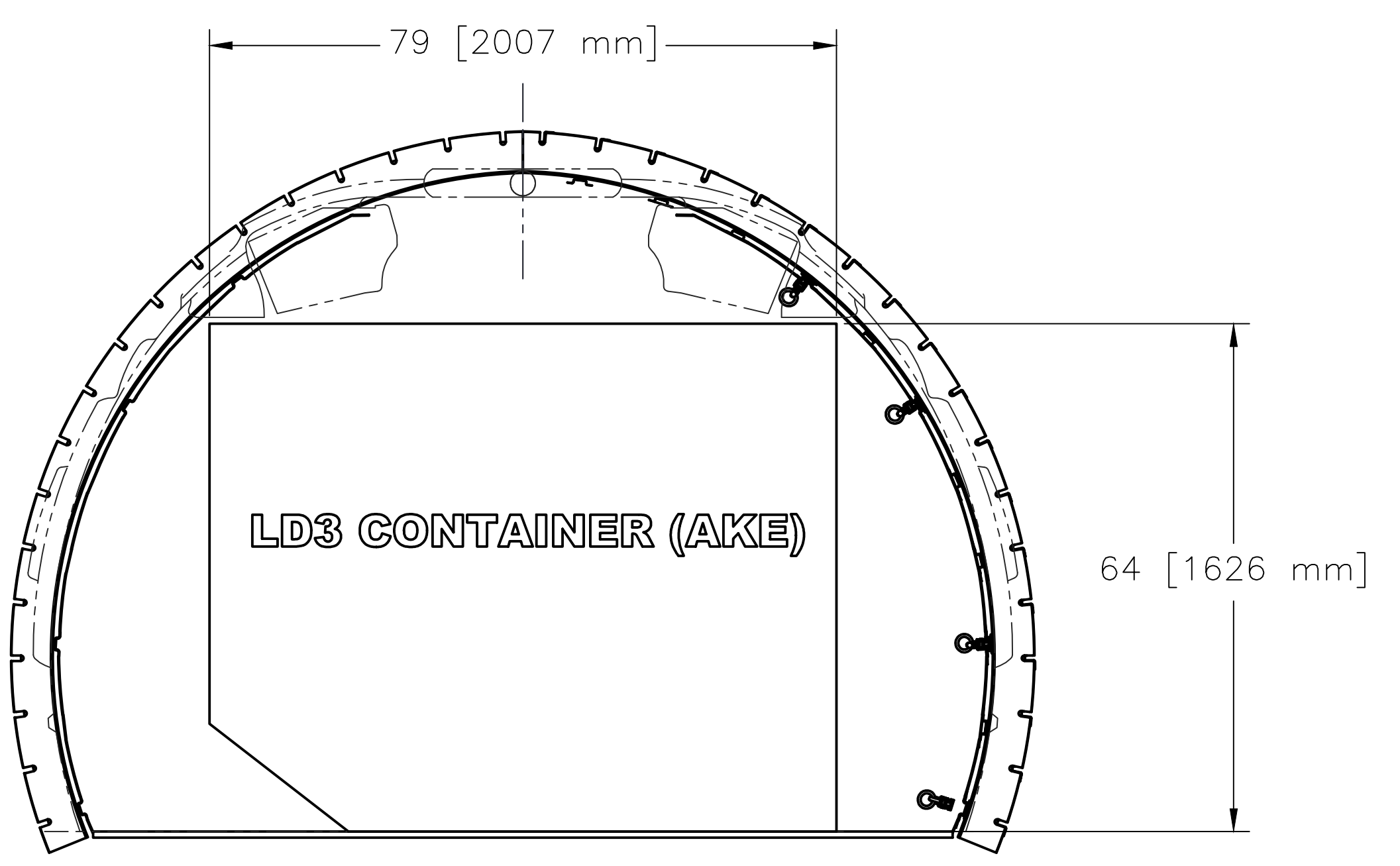
VIEW A-A FUSELAGE CROSS SECTION
